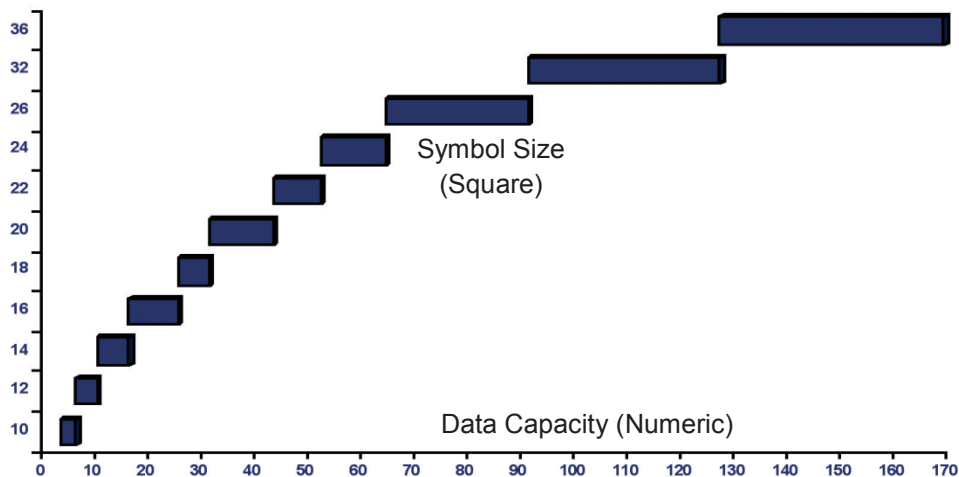
Figure 1-3 Symbol Size vs. Numeric Capacity
